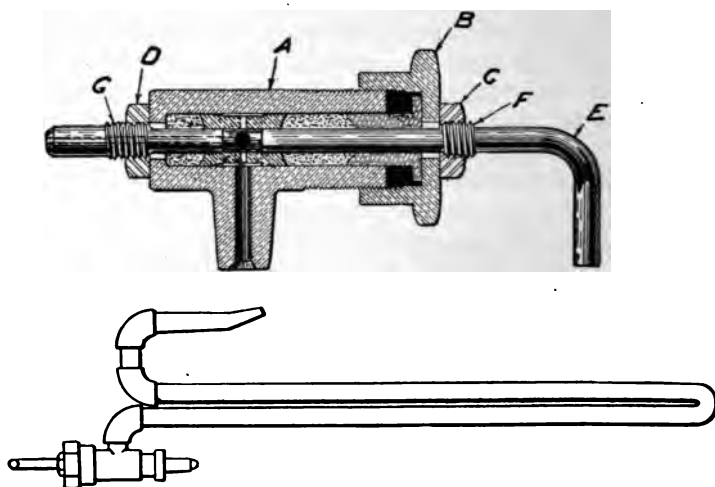
FIG. 366.—Usual pattern of "torch" head and starting "torch," used on several American steam carriages. The head parts are lettered as follows: A, body of head; B, threaded cap; C and D, nuts working on screws, F and G, on rod, E. Screw, G, gives attachment to the collar on the valve stem, as shown at B, in the succeeding figure.
